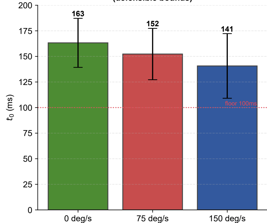
C. HRT non-decision time (defensible bounds)
