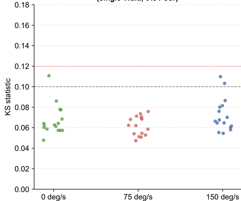
A. HRT fit quality (single-Wald, 0% Poor)
