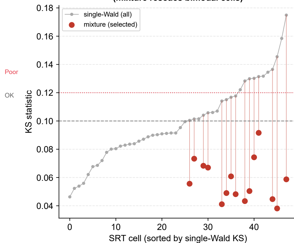
B. SRT fit quality (mixture rescues bimodal cells)
